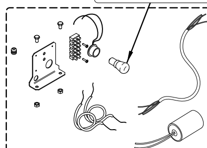
cod. 933130P piastrina porta lampada lamp support support lampe soporte bombilla suporte lâmpada
